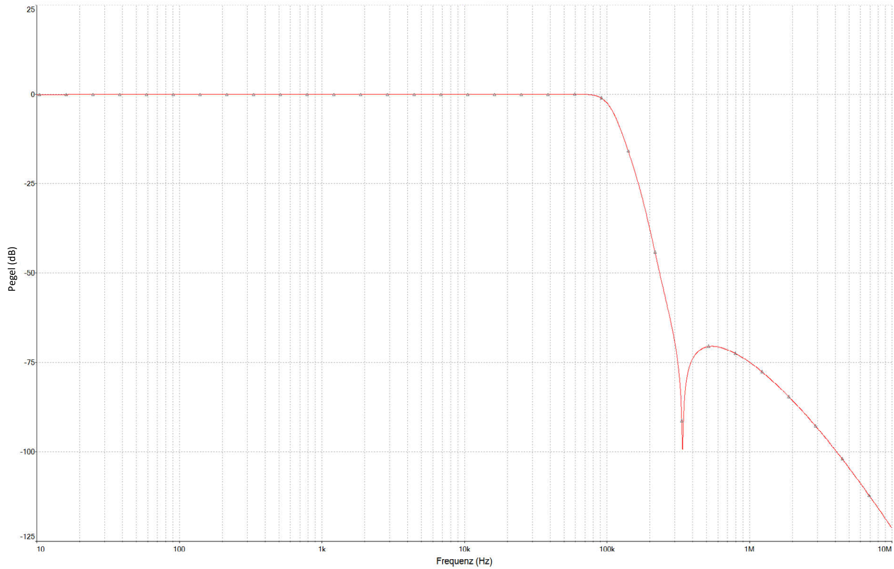
Frequency Response Class-D Measuring Filter
